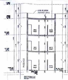
SECTION X-X SECTION
